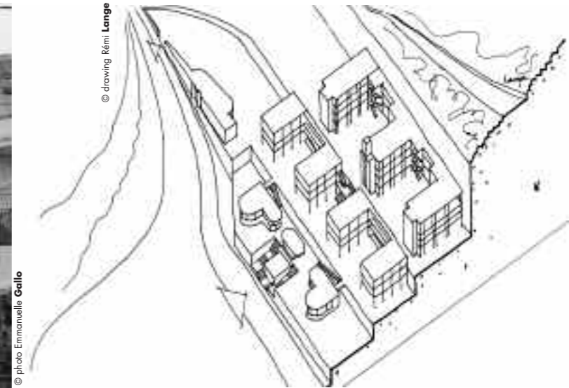
Fig. 3. Lycée Schœlcher, axonometric view
